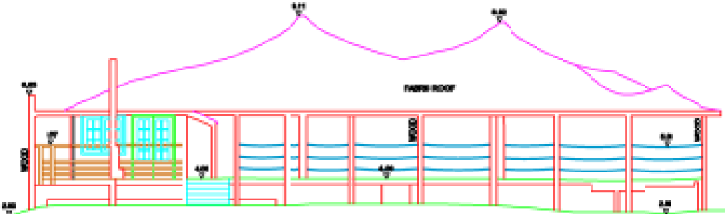
SOUTH ELEVATION
